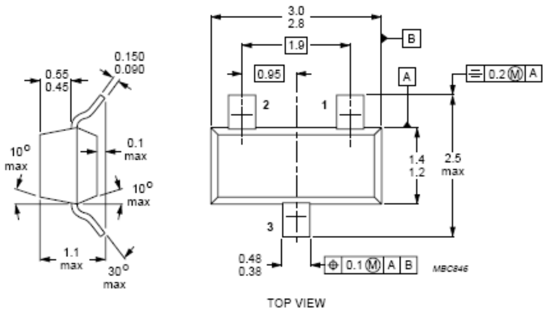
Outline of the KTY82 (SOT23)
